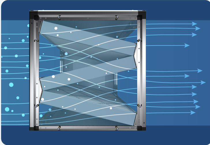
Premium high MERV filtration that meets restrictive SEER 2 requirements. Designed to optimize airflow and pressure drop, while impressive MERV 16 filtration effectively traps particles as tiny as 0.3 microns.
